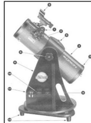
Orion StarBlast Telescope
